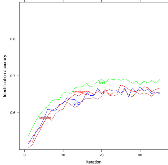
Figure 3: Identification accuracy between connected agents for communities of different network structures.
